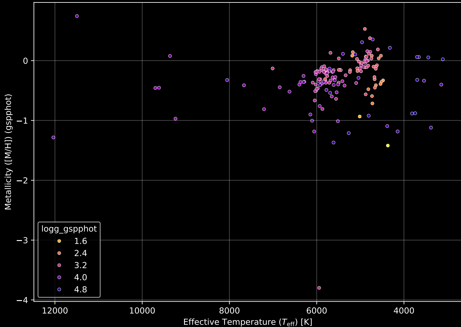
APOGEE DR17 Field: [K2_C11_355+09_btx] Stellar Population Parameters (n= 161)
