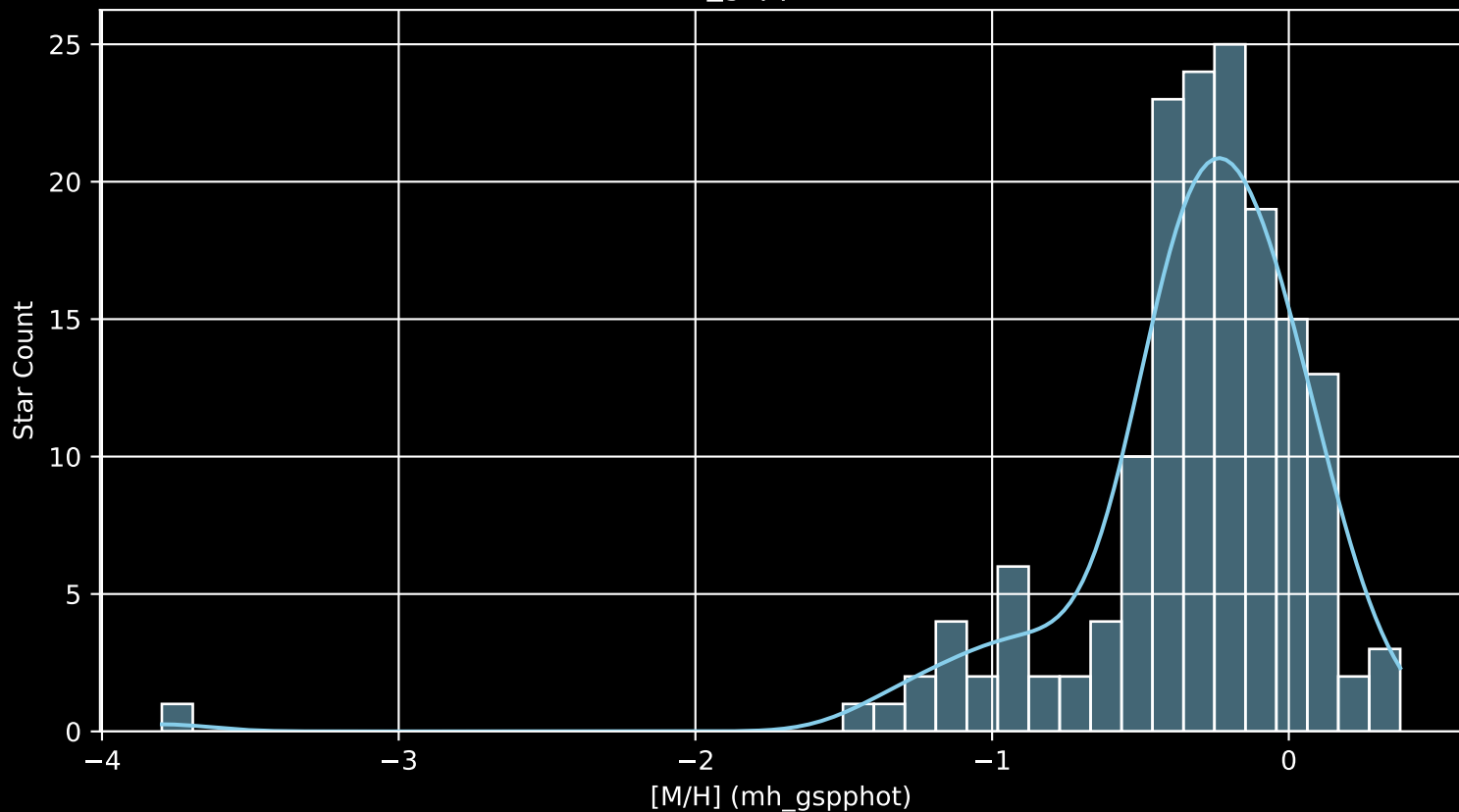
APOGEE DR17 Field: [K2_C11_355+09_btx [M/H] (mh_gspphot) (n= 159)
