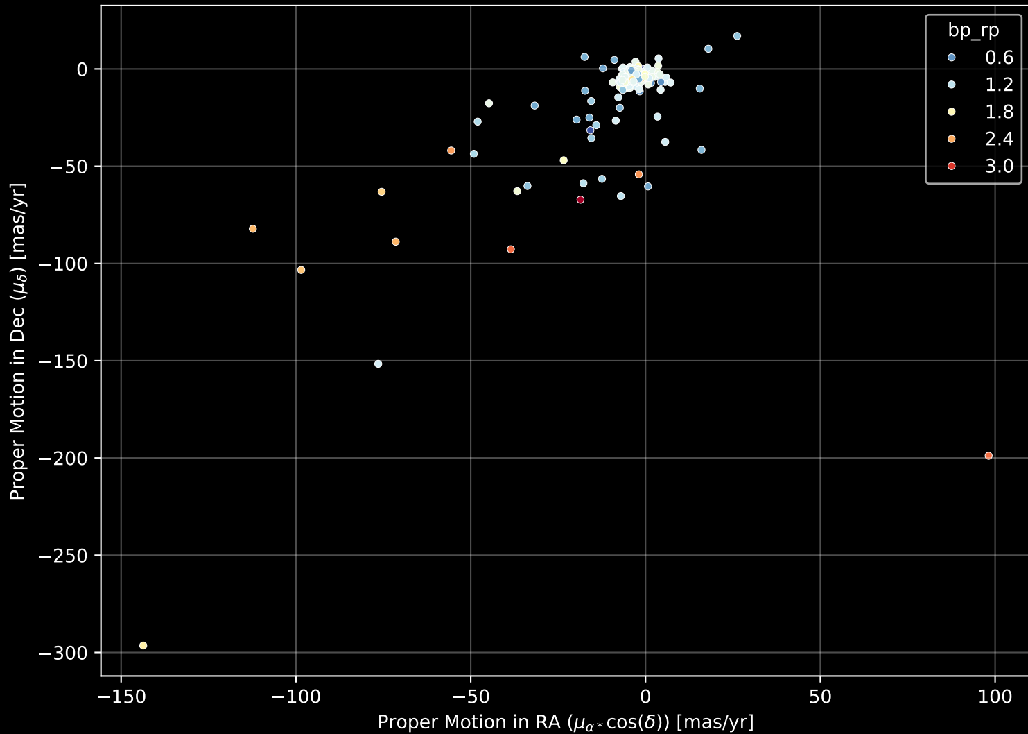
APOGEE DR17 Field: [K2_C11_355+09_btx] Proper Motion Diagram (n= 161)
