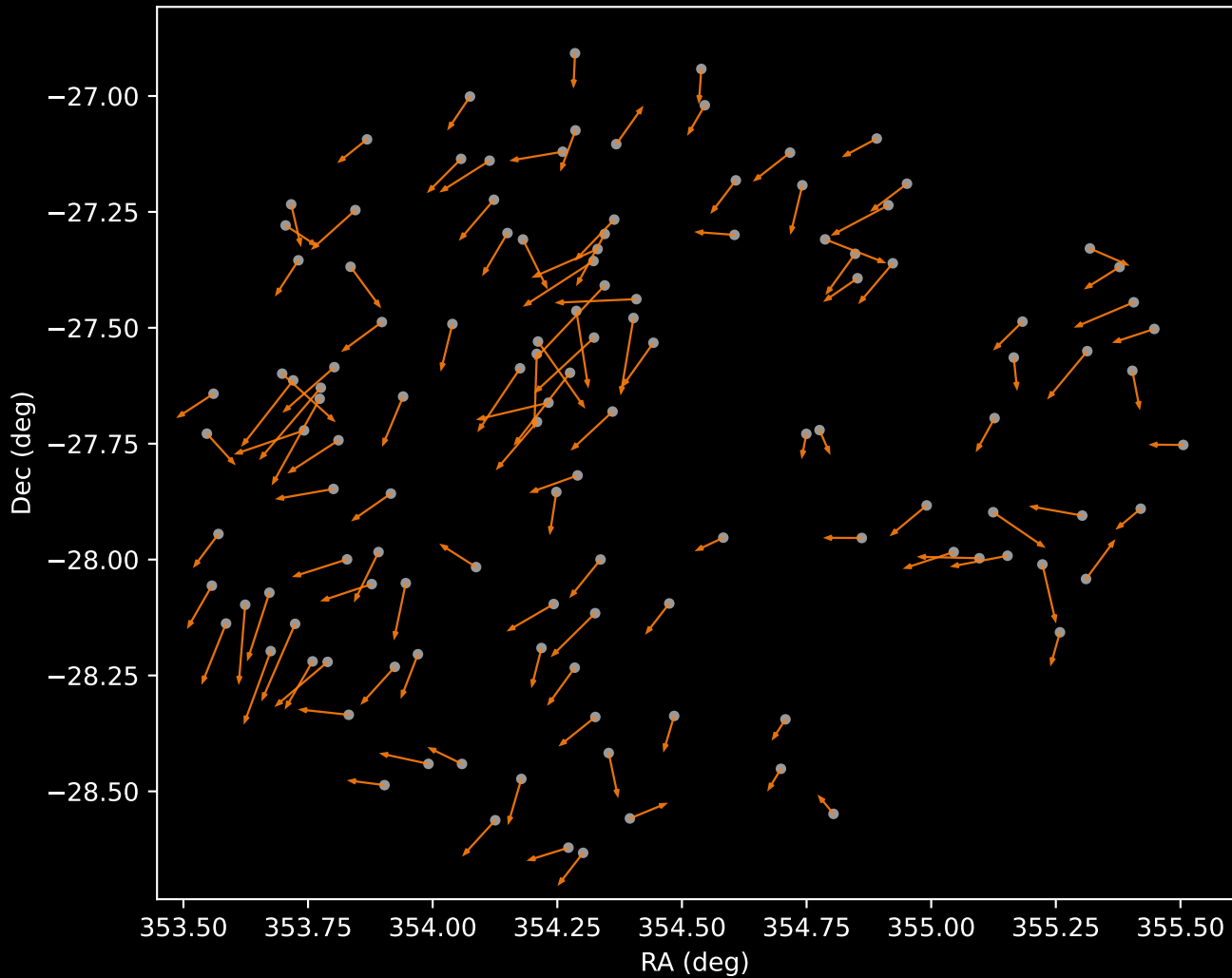
APOGEE DR17 Cluster 2 Proper Motion Vectors (n=123)
