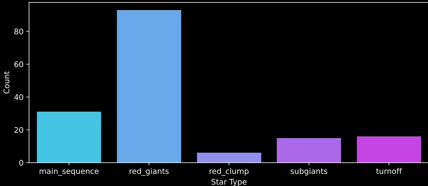
APOGEE DR17 Field: [K2_C11_355+09_btx] Count plot of Star Type
