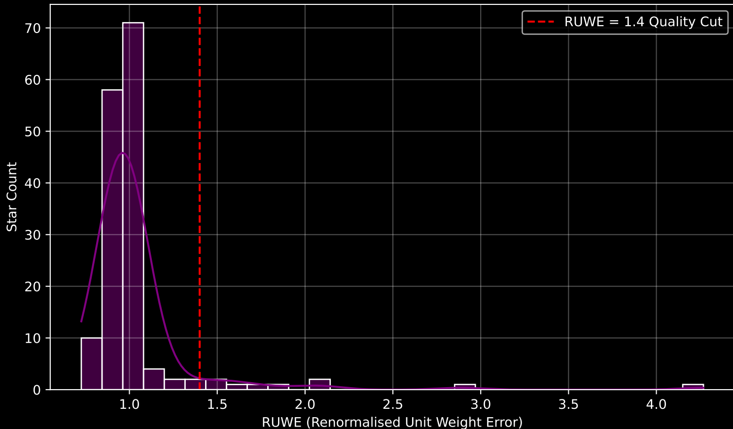
GAPOGEE DR17 Field [K2_C11_355+09_btx] RUWE Distribution (n= 156)
