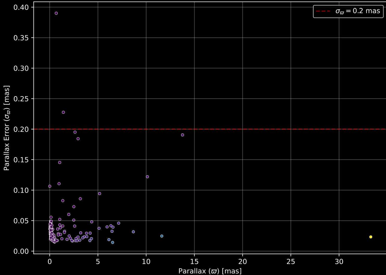
APOGEE DR17 Field: [K2_C11_355+09_btx] Parallax Quality (n= 161)
