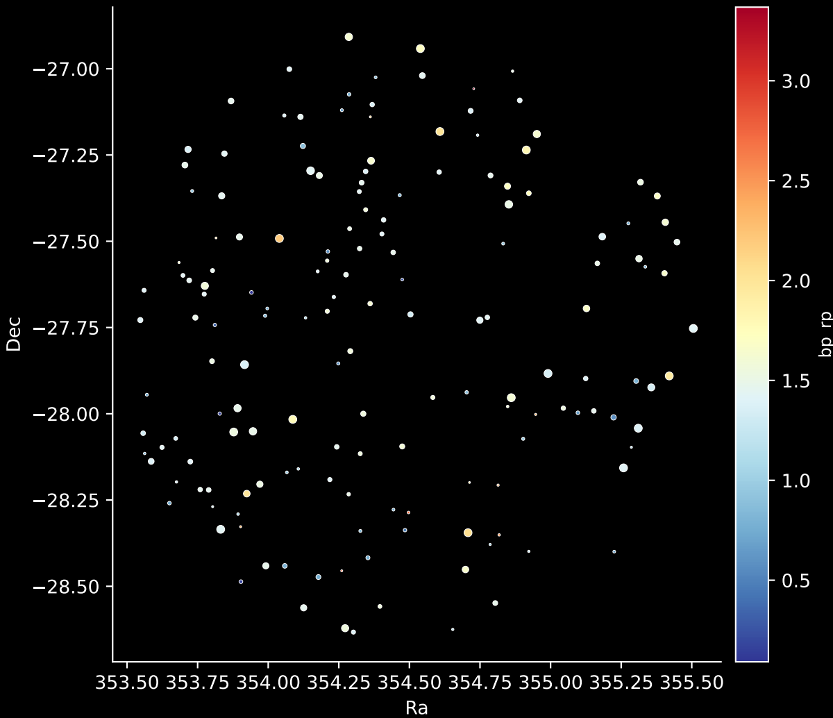
APOGEE DR17 Field: [K2_C11_355+09_btx] Stars: 161
